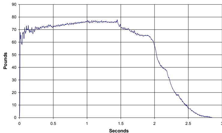
Aerotech J270W-14A DMS
