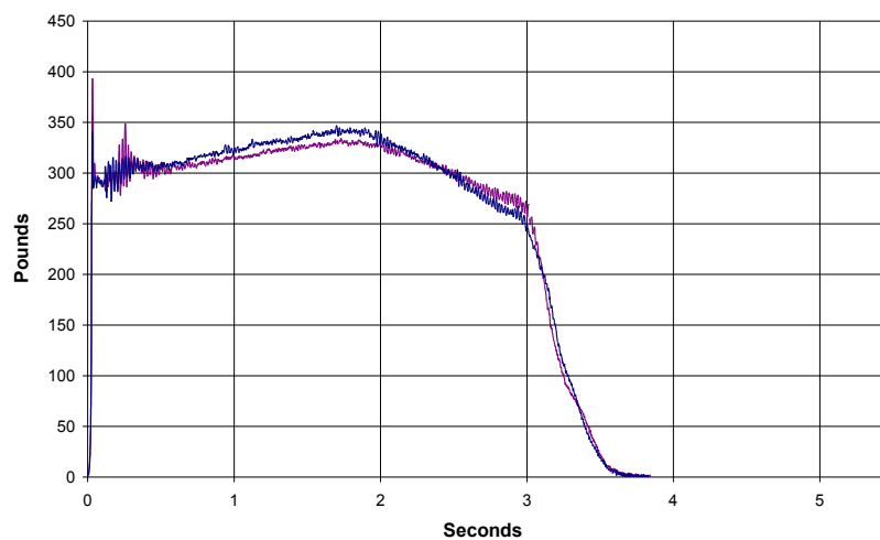
Aerotech L1250DM
