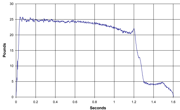
Aerotech G80NT-10A DMS
